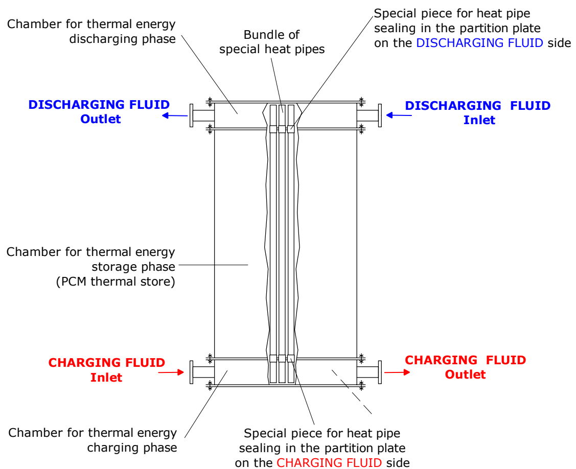
Side view of the PCM thermal energy storage heat pipe based system
